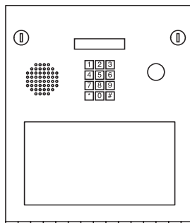
1810 Flush 12" W x 13.5" H x 2.5" D 30.4cm W x 34.3cm H x 6.35cm D
